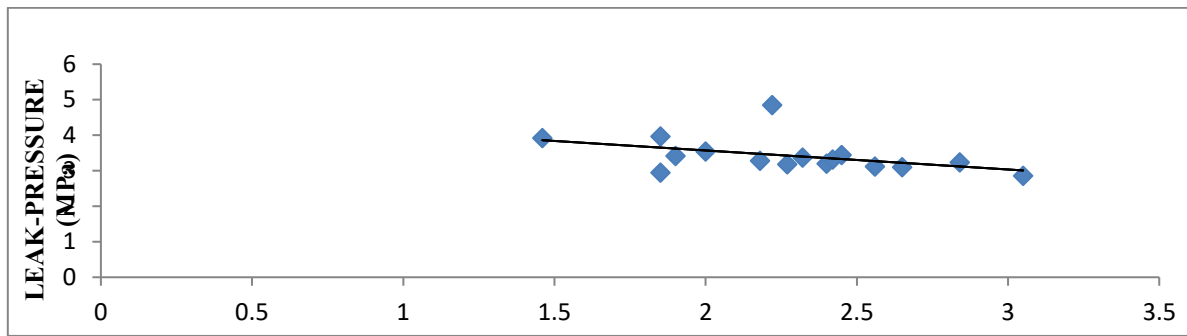
Figure 4: linear relationship between leak pressure and porosity.
