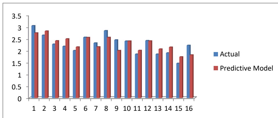
Figure 1: Chart of porosity correlation between experimental and predictive model values.
