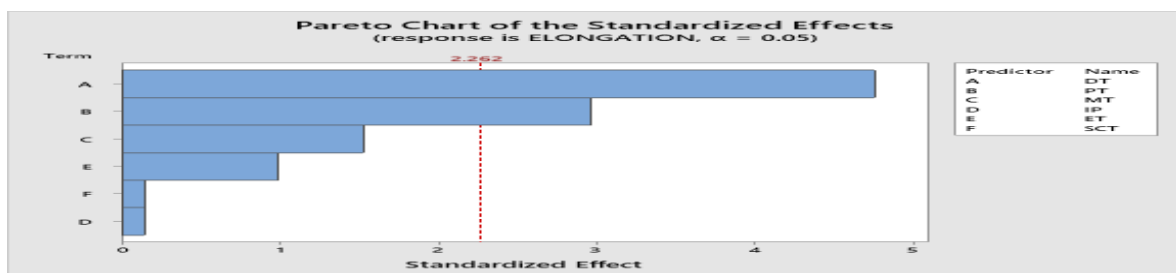
Figure 6: Plot showing influence of process parameters on elongation as response factor
