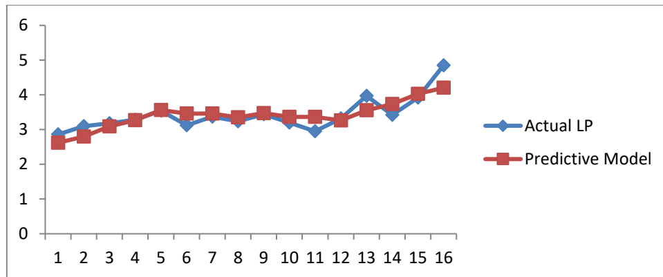
Figure 2: Plot of Leak-pressure correlation between experimental and predictive model values
