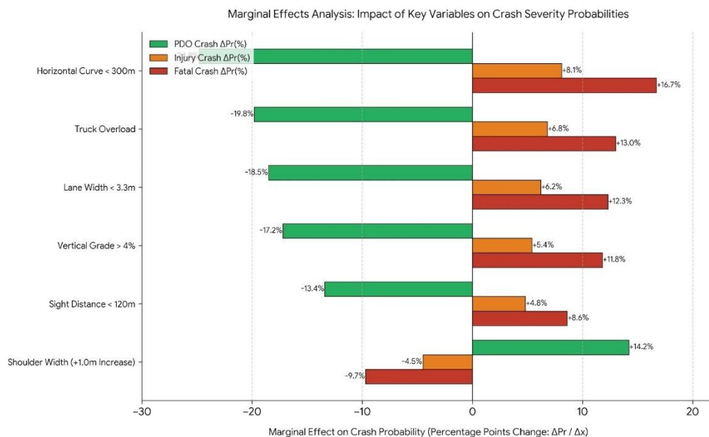
Fig. 1.2: Marginal Effect of Key Geometric Variables on Severe Truck Crash Probability (Mixed Logit Model)
